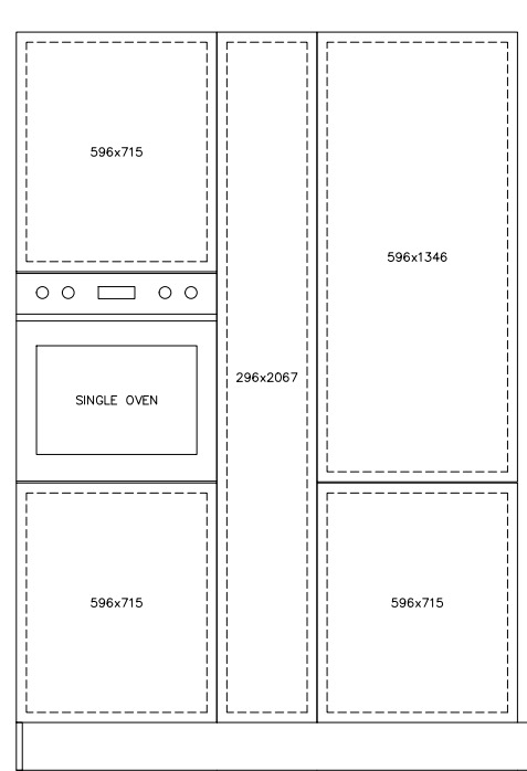
4 KITCHEN ELEVATION
