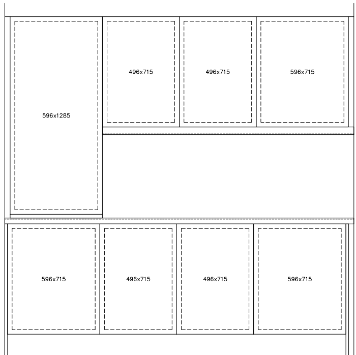
1 UTILITY ELEVATION
