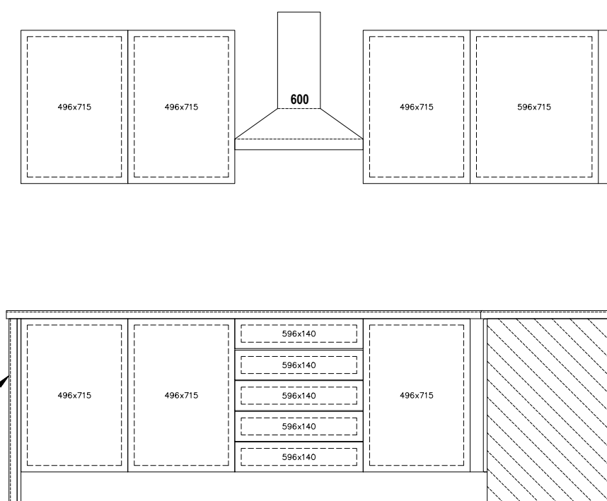
2 KITCHEN ELEVATION
